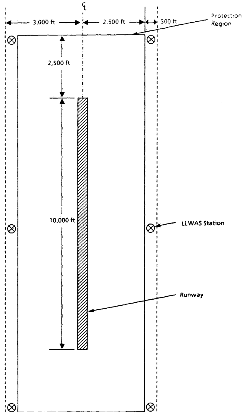
FIGURE 2-1. IDEAL GEOMETRY FOR THE DETECTION OF MICROBURST WINDSHEAR ALONG A RUNWAY
