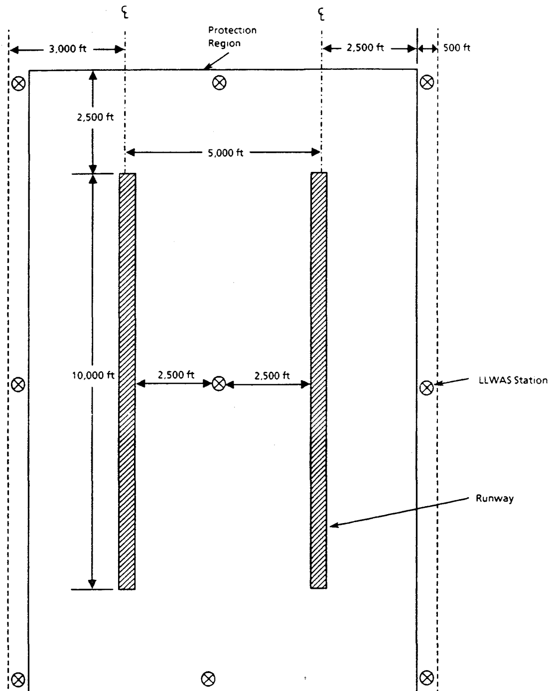
FIGURE 2-8. PROTECTING PARALLEL RUNWAYS
